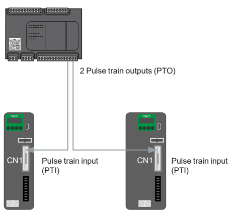
Easy Lexium 16 servo drives controlled by Easy Modicon M200 logic controller
