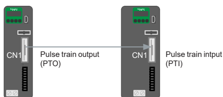
Easy Lexium 16 drive controlling another Easy Lexium 16 drive
